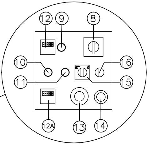
PANNELLO COMANDI CONTROL PANEL
